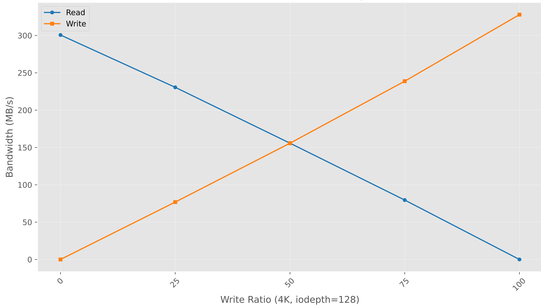
Bandwidth vs Write Ratio (4K, iodepth=128)
